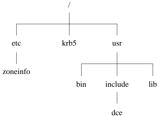
Figure B-3 shows the directories that DCE uses in the standard UNIX tree. Figure B-3. Standard UNIX Directories Tree
