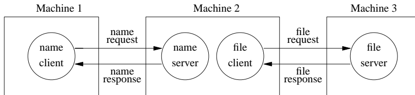
Figure 1–1. Interaction of Clients and Servers
