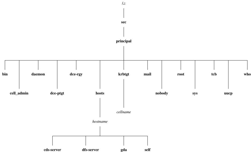
Figure A-6. The sec/principal Directory
