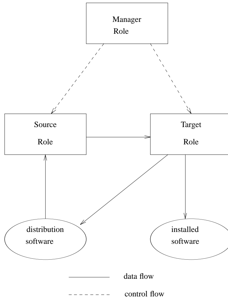
Figure 1-1 POSIX 1387.2 Distributed Roles
