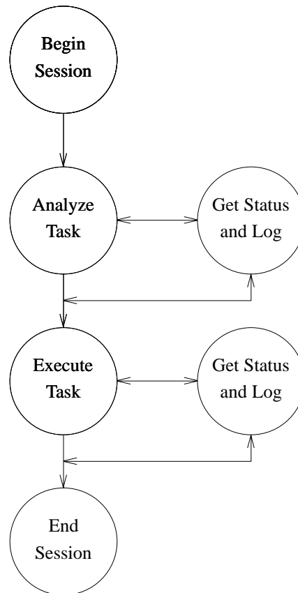
Figure 2-4 XDSA-DCE Status and Log Retrieval
