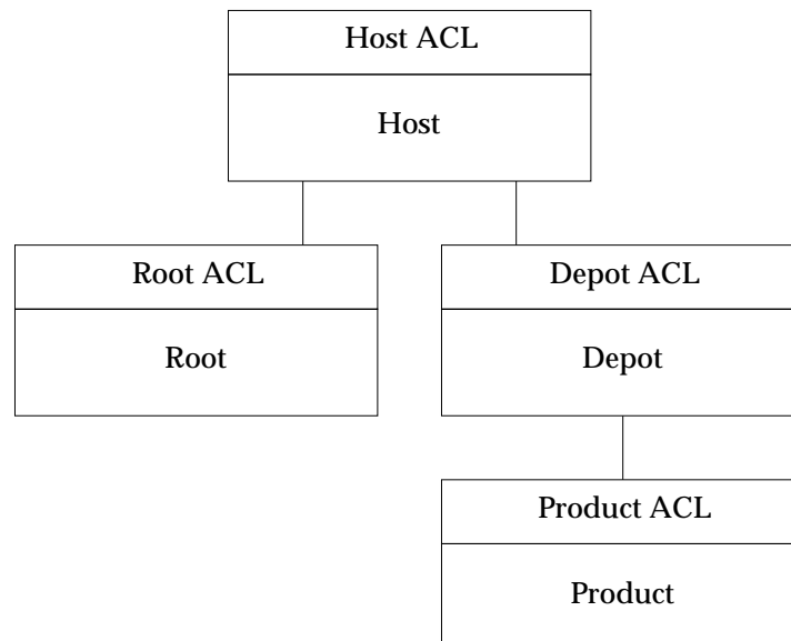
Figure 8-1 ACL Object Types
