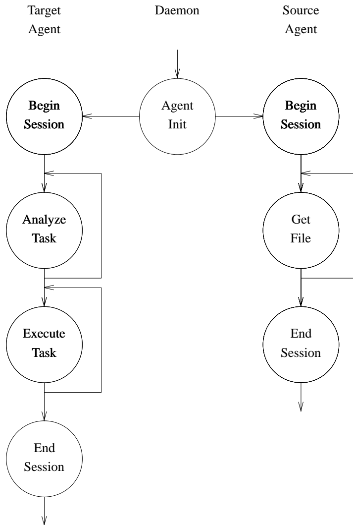
Figure 2-3 XDSA-DCE Target and Source Sessions
